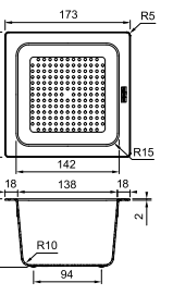
Small strainer bowl
