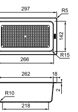
Large strainer bowl
